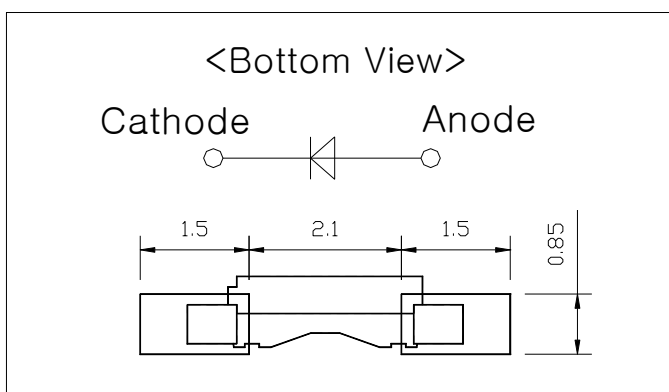
Recommended solder Pattern
